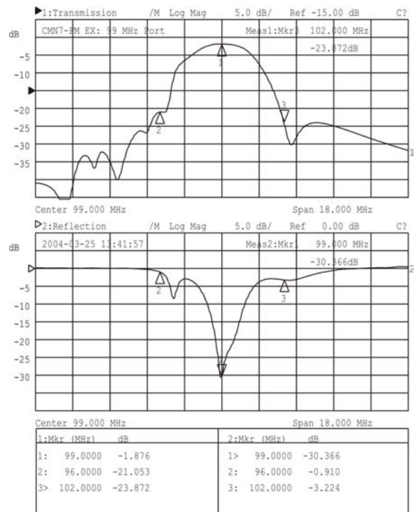
Fig. 1 Typical Frequency response of filtered FM input.
